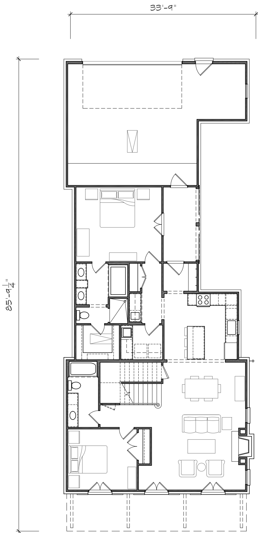
FIRST FLOOR
